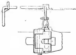
Fig. 2199. End Elevation.
